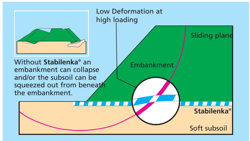
Embankments with Stabilenka® remain stable. Details shows fabric deformation during initial loadings.
