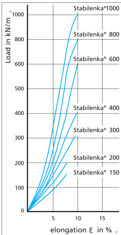
Load-elongation curve of Stabilenka® standard types
